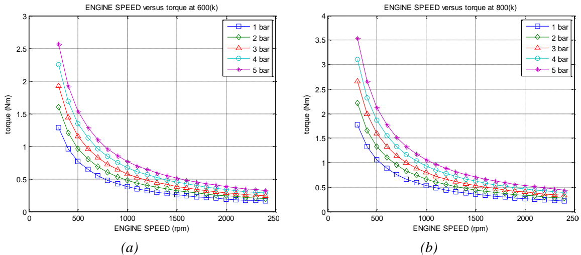
Figure 7. Torques versus engine speeds for various applied pressures at (a) T_h=600\text{ K} and (b) T_h= 800\text{ K} .
